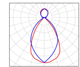
UGR19 REFLECTOR 65° incl. indirect light module
