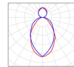
UGR22 MICROPRISMATIC incl. indirect light module
