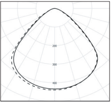
Lichtkurven | Lightcurves
