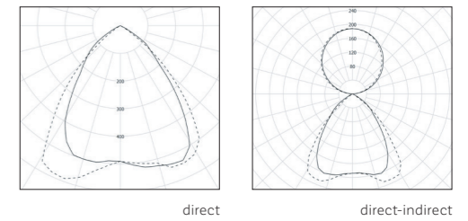
Lichtkurven | Lightcurves
