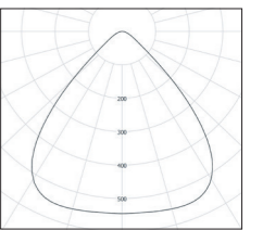
UGR<26 medium 90°
